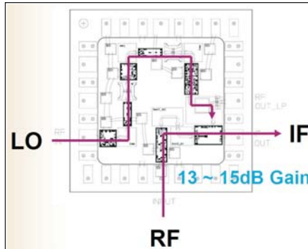
Figure 7 . Outline of signal paths within the package.
